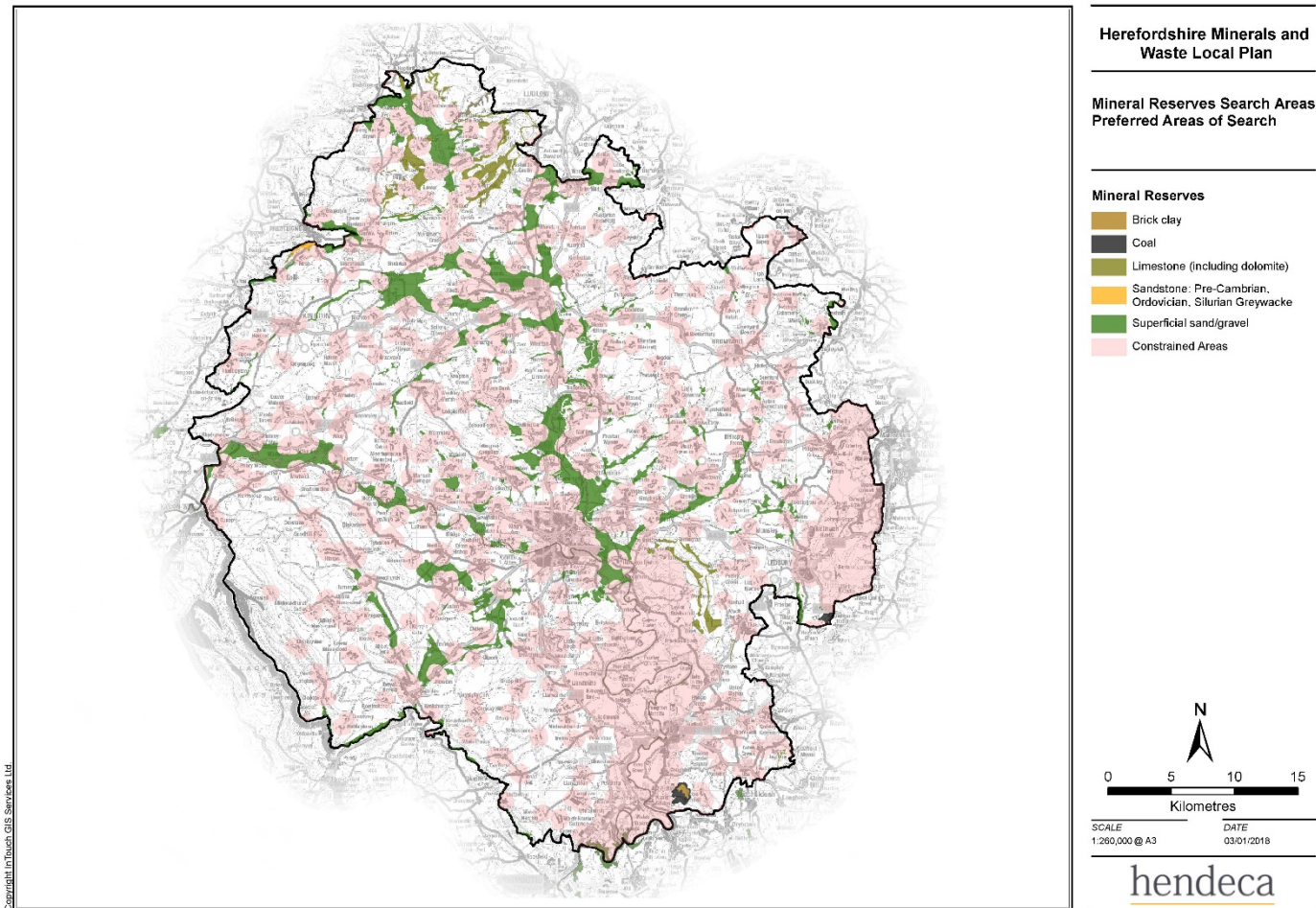
Figure 2.5 Areas of search in Herefordshire
