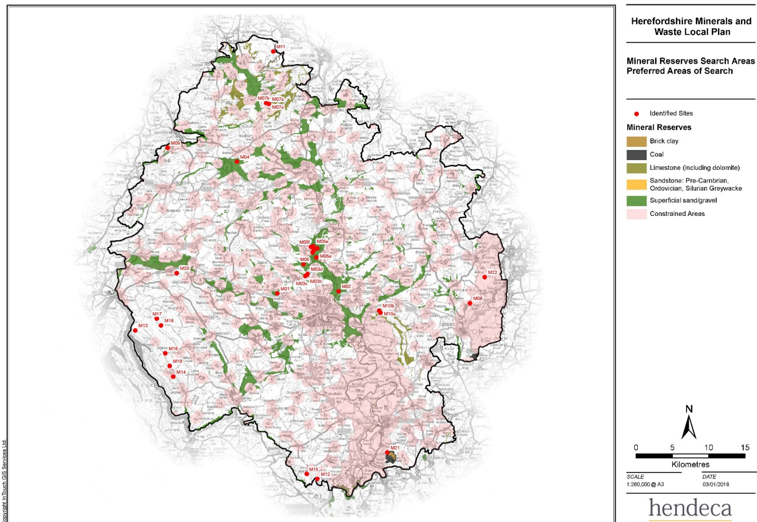
Figure 2.6 Areas of search in Herefordshire, with identified sites
