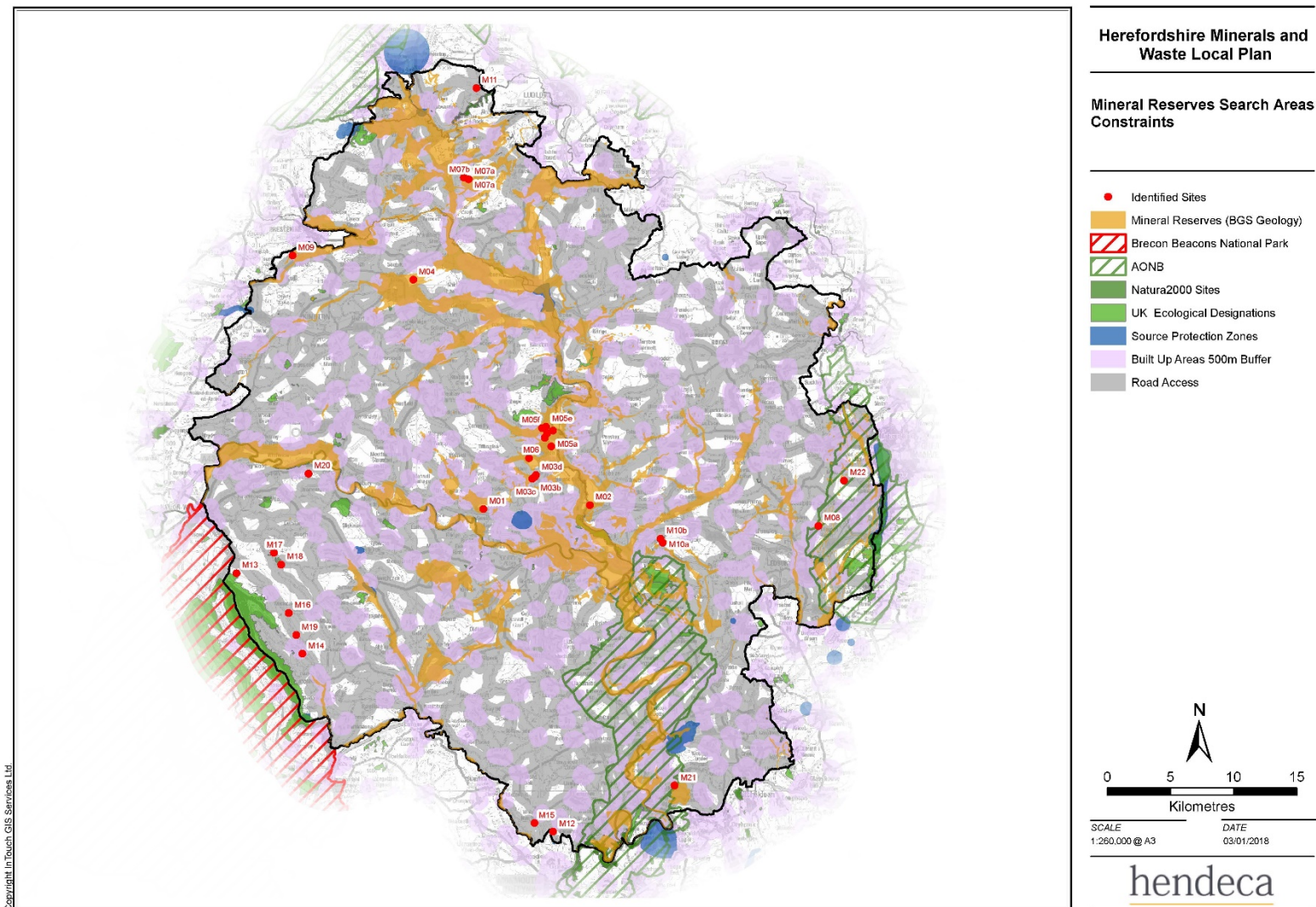
Figure 2.4 Data layers applied to minerals resource mapping, with identified sites
