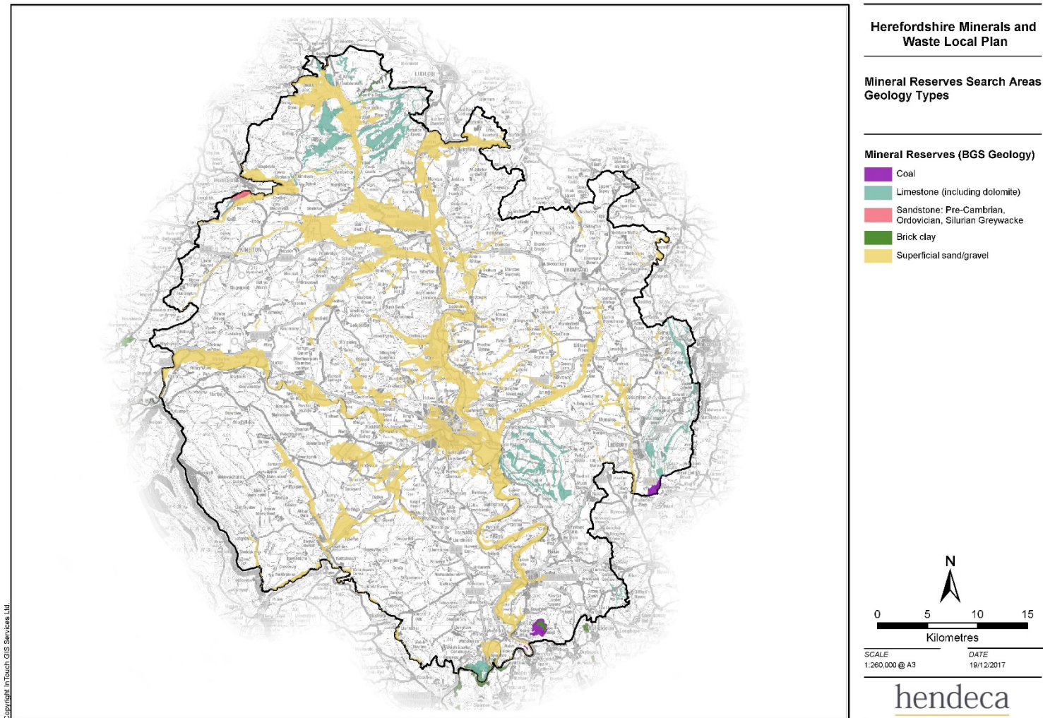
Figure 2.1 Minerals resources in Herefordshire, British Geological Survey
