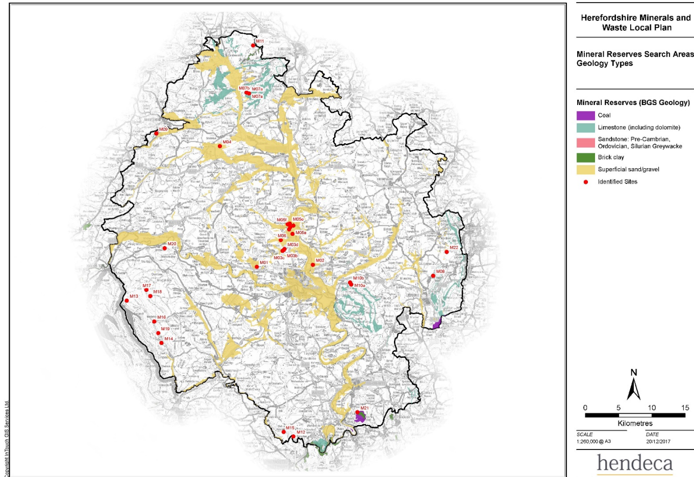
Figure 2.2 Minerals resources in Herefordshire, British Geological Survey, with identified sites
