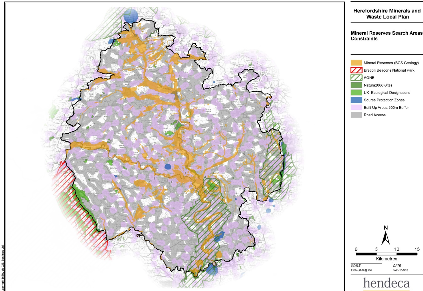
Figure 2.3 Data layers applied to minerals resource mapping
